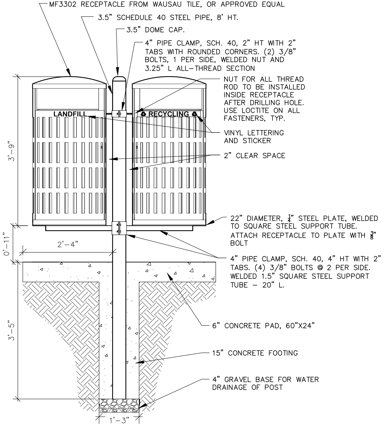
STANDARD DUAL BIN CONFIGURATION
