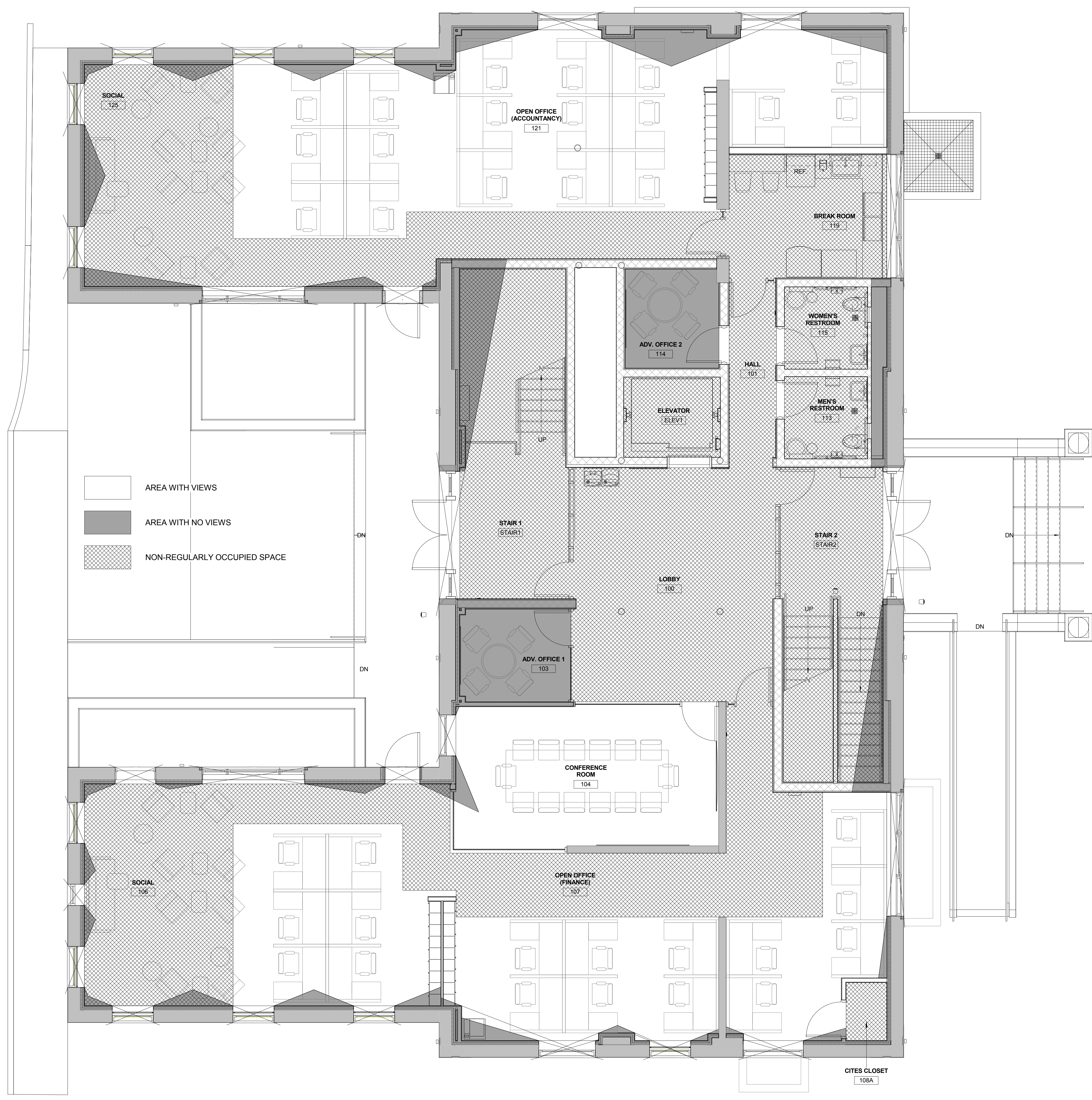
NORTH FIRST FLOOR LEED IEQ 8.2 - Views 1/4" = 1'-0"
