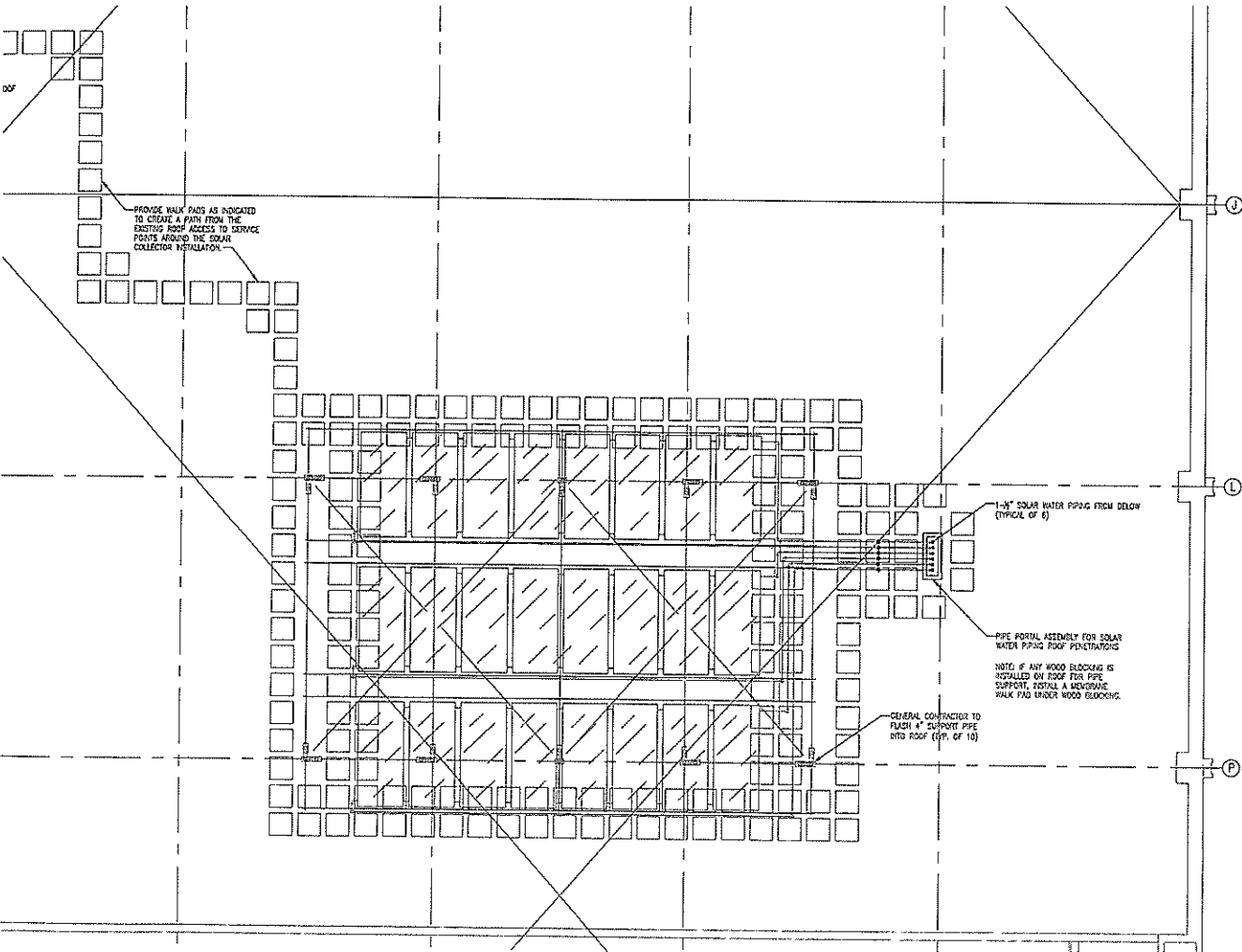
1 PARTIAL ROOF PLAN - ROOFING SCALE: 1/4" = 1'-0" NORTH
