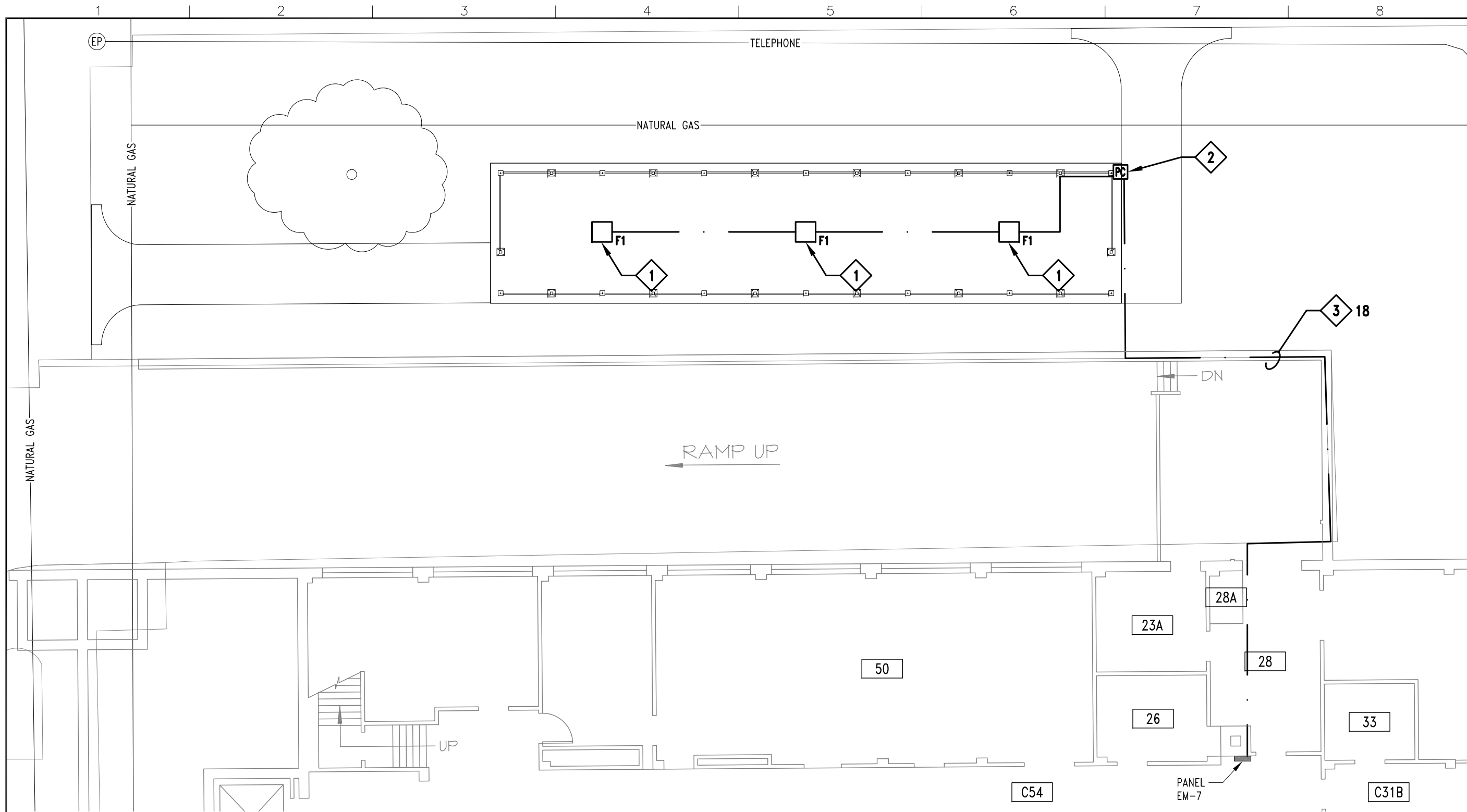
A ELECTRICAL PLAN NORTH SCALE: 1" = 10'
